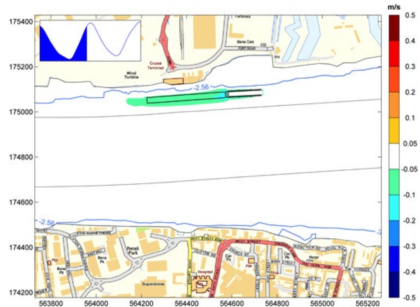
Figure 17.32: Essex Project Site difference in current magnitude at time of peak flood tide against the baseline model.
